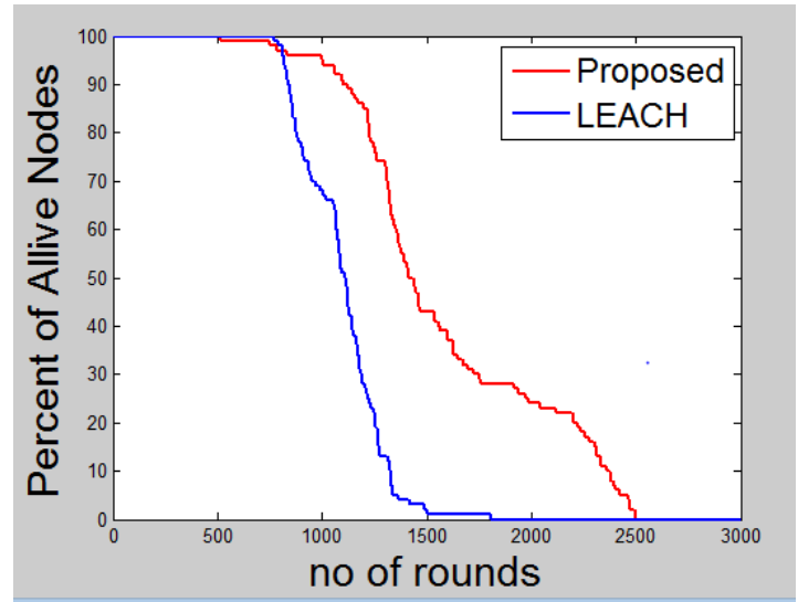
Fig. 5 Percentage of alive nodes in each round
