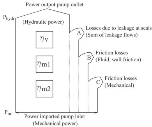
Fig.1 Block diagram showing different losses.
