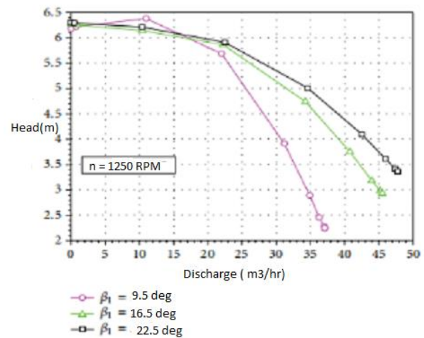
Figure 7: The graph of total head as verses flow rate (discharge), studying the non cavitating performance.
