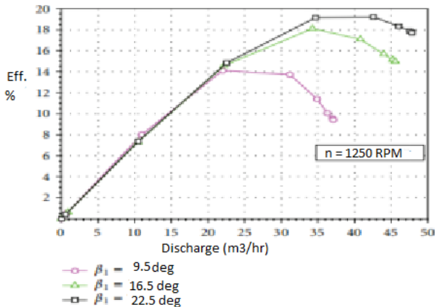
Figure 8: The graph of efficiency verses flow rate (discharge) , studying the non Cavitation performance.
