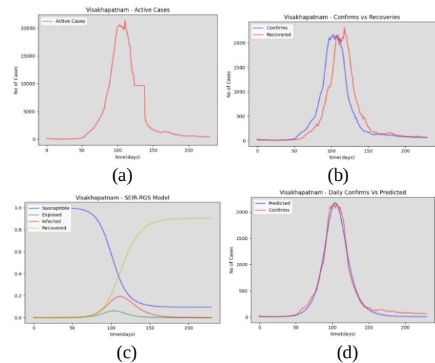
Fig 15: Visakhapatnam district (a) daily active cases (b) confirms vs recoveries (c) SEIR-RGS model results (d) daily confirms vs predicted by proposed SEIR-RGS model
