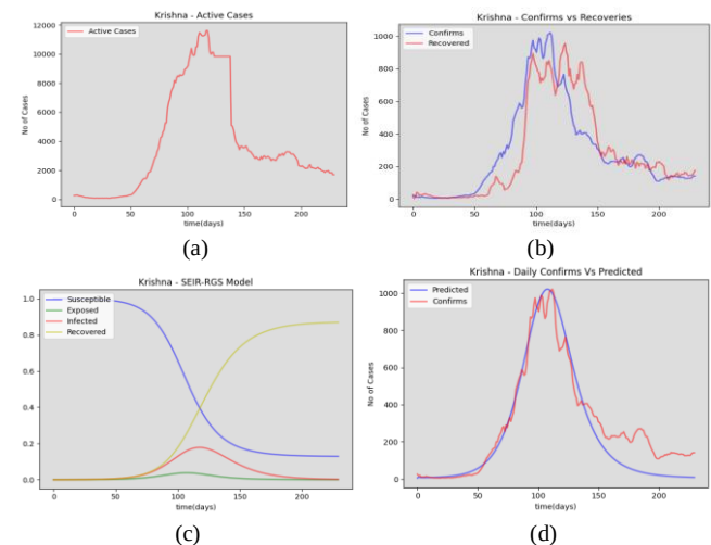
Fig 10: Krishna district (a) daily active cases (b) confirms vs recoveries (c) SEIR-RGS model results (d) daily confirms vs predicted by proposed SEIR-RGS model
