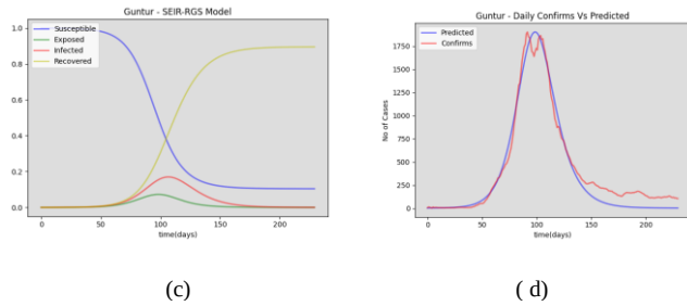
Fig. 8: Guntur district (a) daily active cases (b) confirms vs recoveries (c) SEIR-RGS model results. (d) daily confirms vs predicted by proposed SEIR-RGS model
