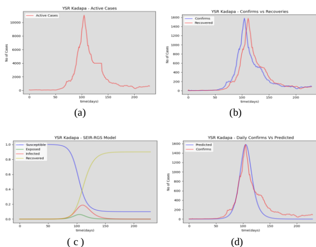
Fig 9: Kadapa district (a) daily active cases (b) confirms vs recoveries (c) SEIR-RGS model results (d) daily confirms vs predicted by proposed SEIR-RGS model
