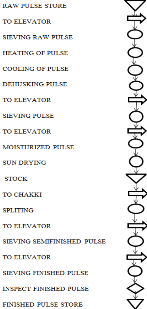
Figure 8: Modify Flow of material
