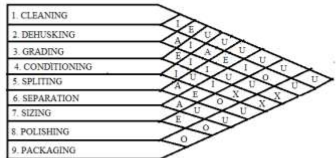
figure 5: Activity Relationship Diagram
