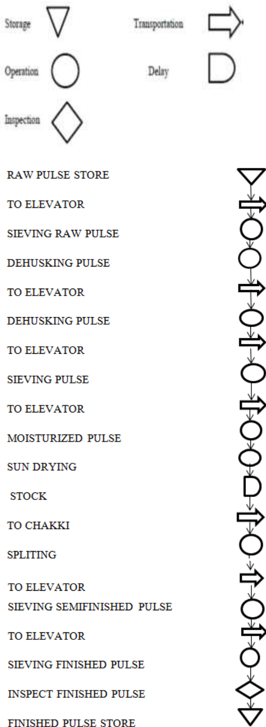
Figure 4: Flow of material in Dal Mill
