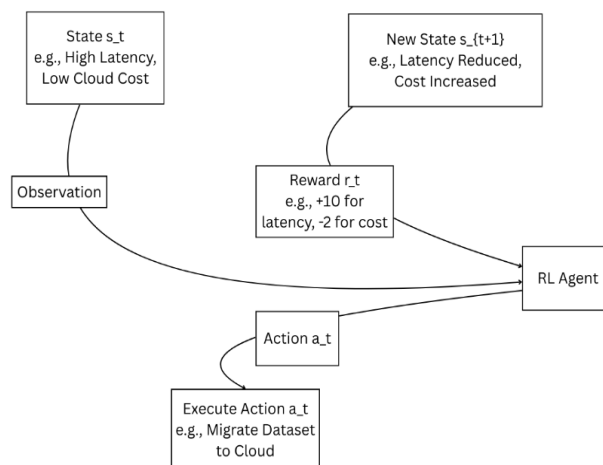
Figure 2. Reinforcement Learning interaction cycle in a hybrid DBMS environment.
