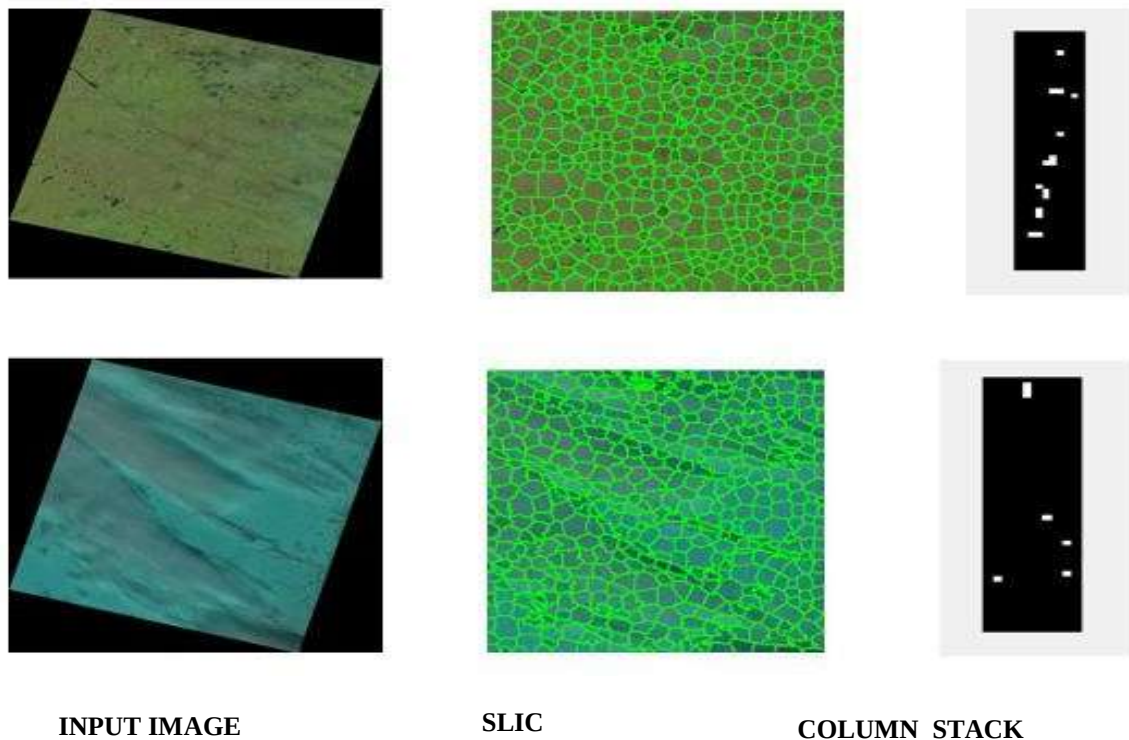
Figure 4.1. Output of SLIC
