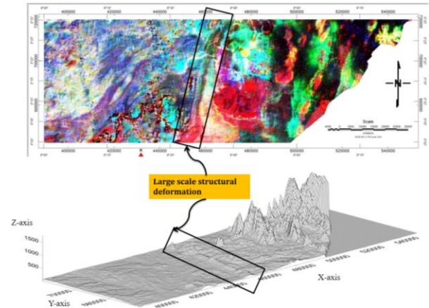
Fig. 11. Large scale structural deformation on both Landsat imagery (at the top) and 3-D structural model (at the bottom).
