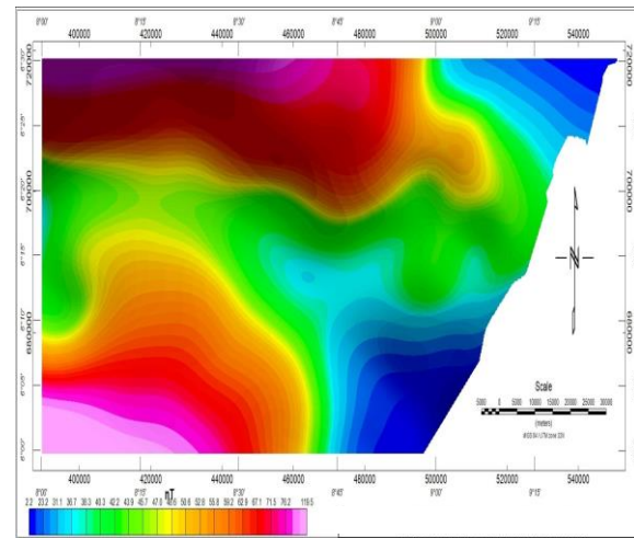
Fig. 4. Regional map of Bamenda Massif
