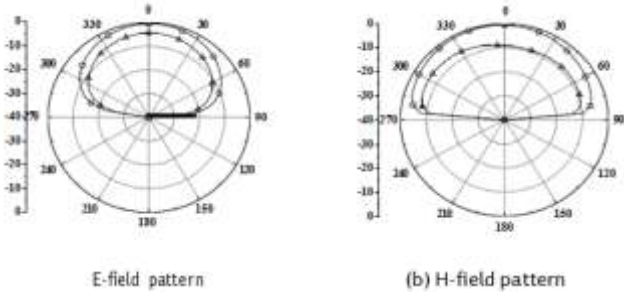
Figure7: Simulated normalize radiation pattern at 3.3 GHz
