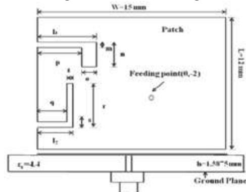
Figure 1: Antenna 1 Configuration
