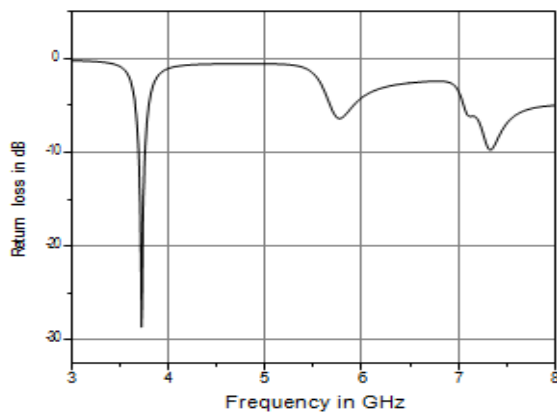
Figure 3: Simulated return loss of the antenna1
