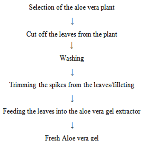
Fig. 3.10 Flow chart for working of hand operated aloe vera gel extractor
