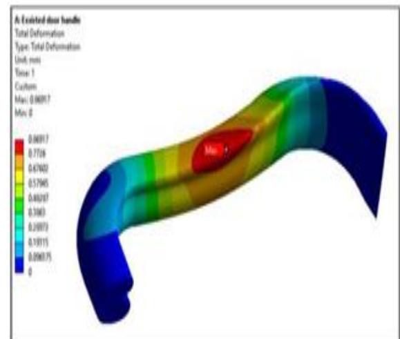
Fig Total Deformation of the handle
