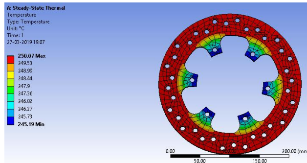
Fig. (a). Temperature of standard disc 1
