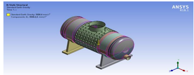
Fig 7 .Gravity loading condition
