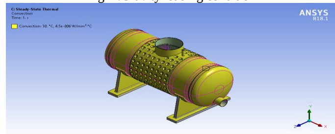
Fig 8 .convection loading condition
