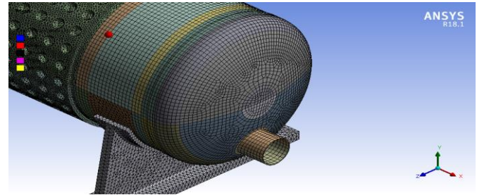
Fig 6 .Hex mesh on vessel
