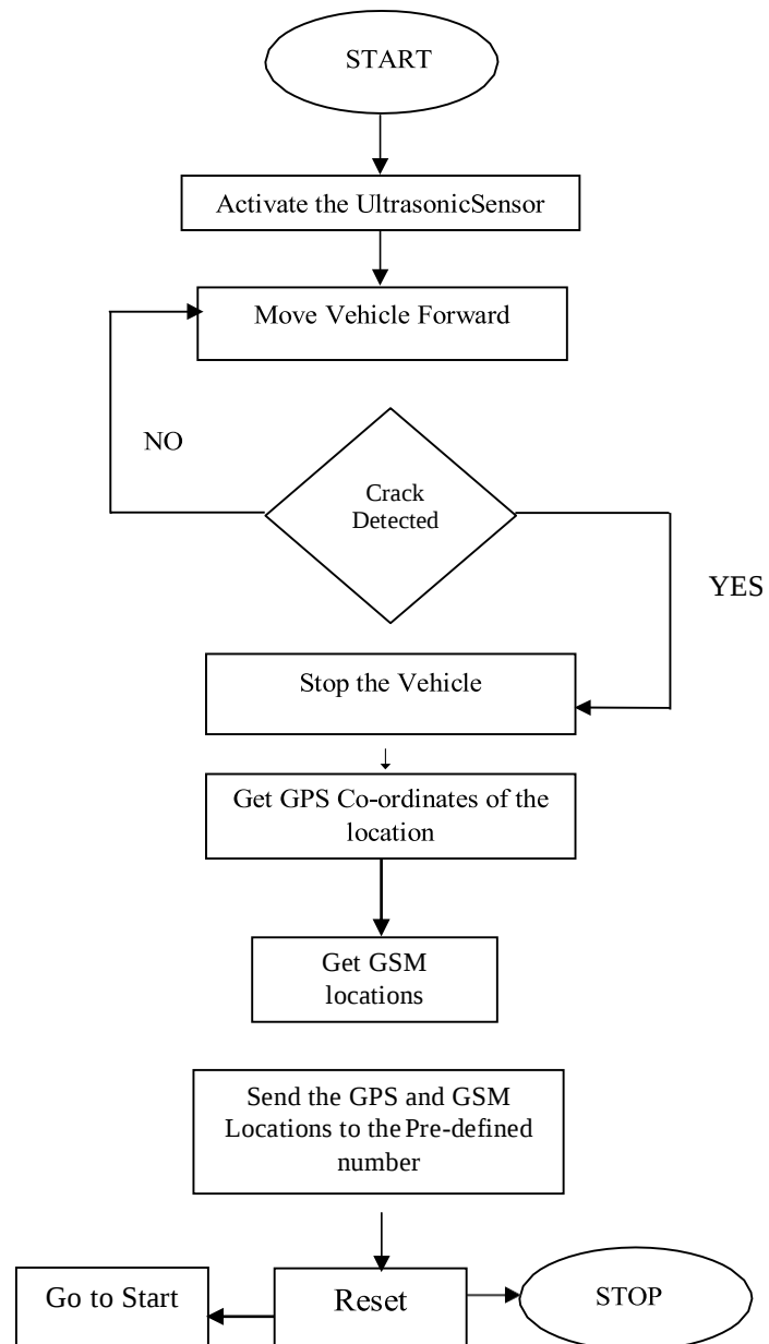
Figure 3: Program Algorithm
