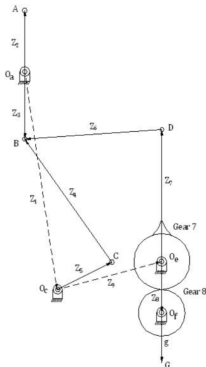
Fig.1 Eight Link Gear Mechanism
