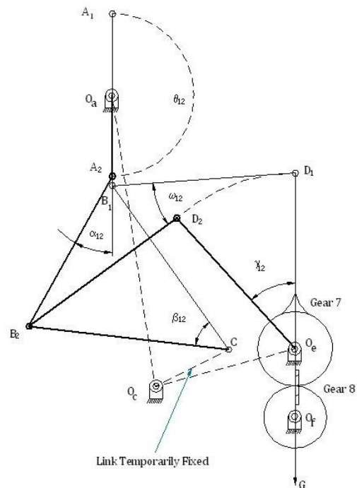
Fig.2 Eight Link Gear Mechanism with Variable Topology Phase I
