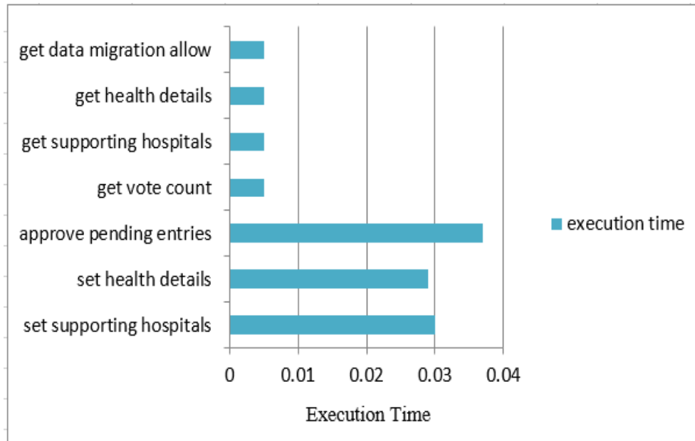
Fig 17: Latency/Execution time
