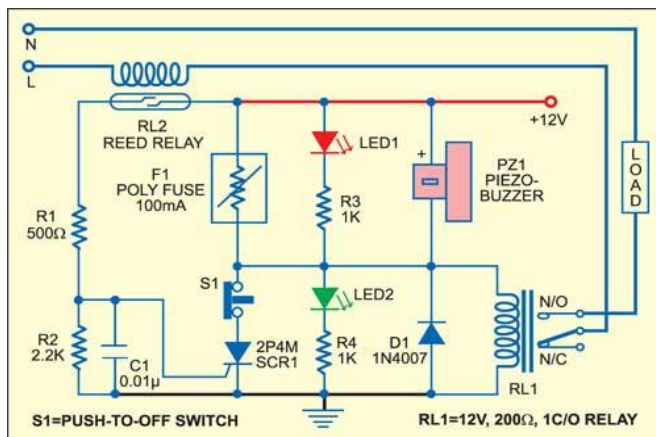
Fig. 2. Complete circuit
