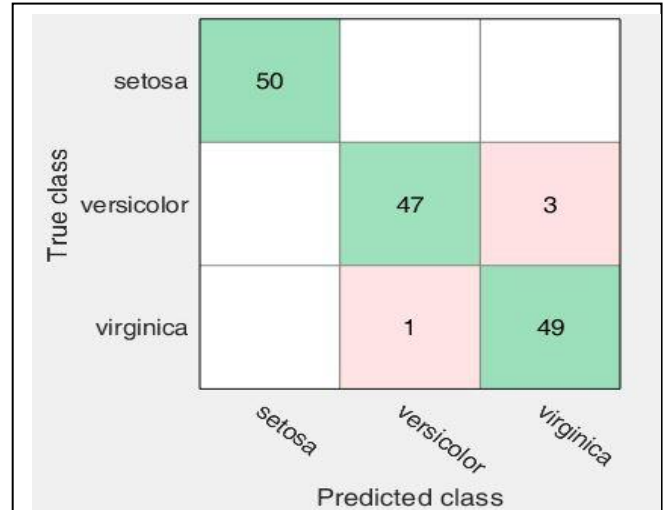
Fig.11. Confusion matrix of LDA with PCA and dimensionality 2.
