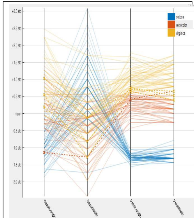
Fig.10. Clustered Fisher Iris Data from LDA with PCA and dimensionality 2 on parallel analysis plot
