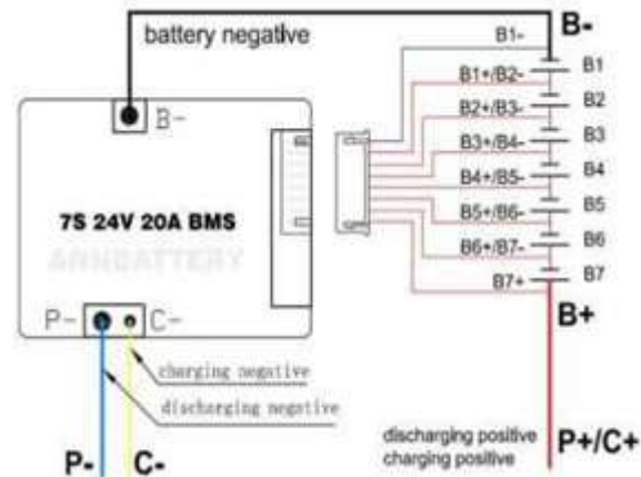
Fig.1. Connection of battery and BMS
