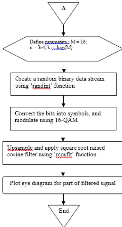
Fig. 6. An Algorithm for Performance Analysis including Filter
