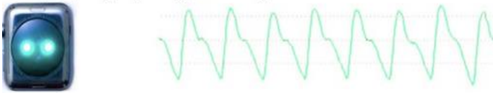
Photoplethysmogram/Tachogram recording
