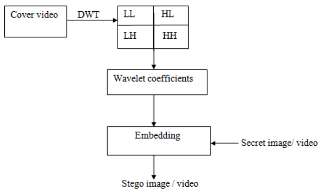
Fig.4: Embedding Process
