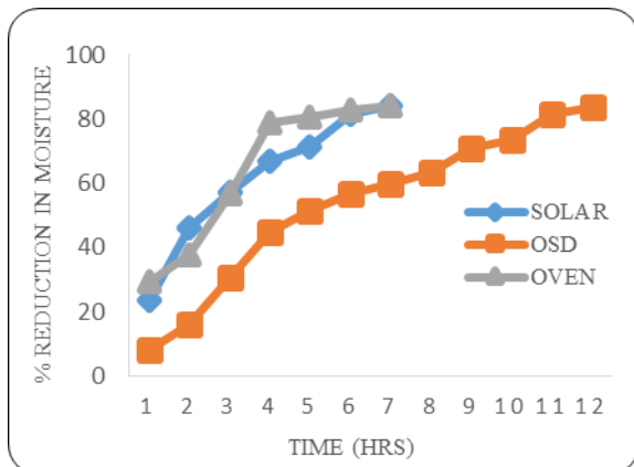
Fig. 5. Time VS % reduction in moisture
