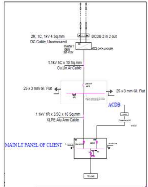
Figure 5: Single Line Diagram of Solar PV Plant
