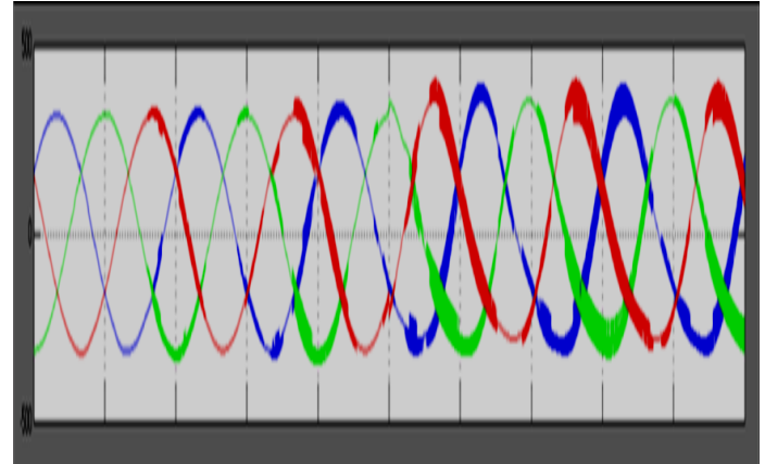
Fig. 6. Load voltage after compensation
