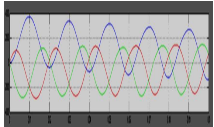
Fig. 7. Load current after compensation
