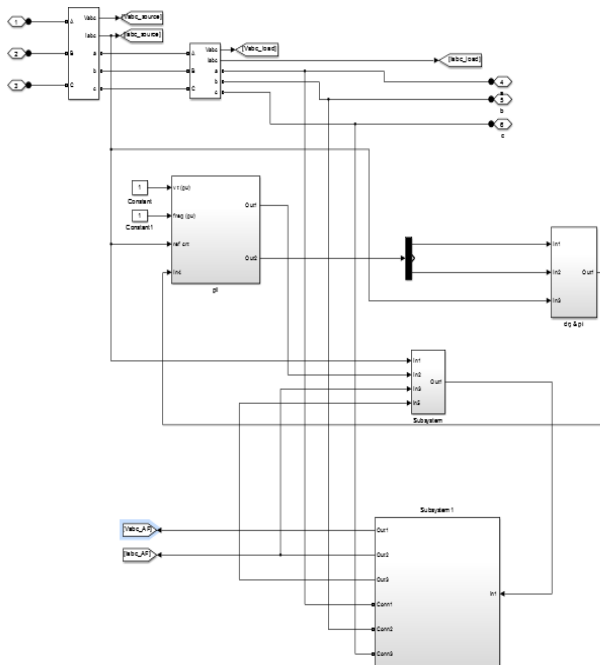
Fig. 3. Simulation of Subsystem with PI-VPI Controller
