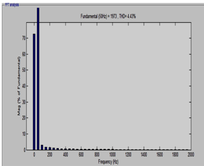
Fig. 10. FFT Analysis
