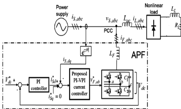
Fig. 1. Block diagram of proposed system with APF
