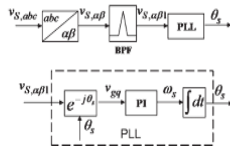
Fig. 4. Block diagram of improved PLL
