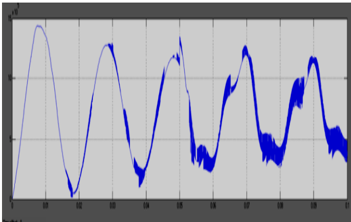
Fig. 9. Reactive power after compensation
