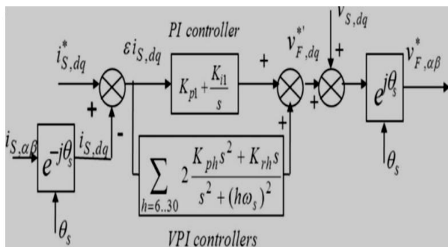
Fig. 5. Block diagram of current controllers
