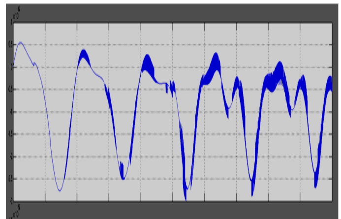
Fig. 8. Real power after compensation
