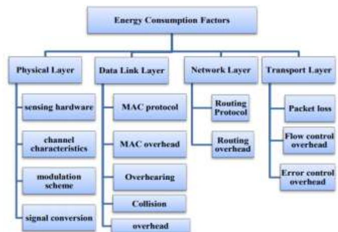
Fig. 1 Energy Consumption Parameters in WSNs
