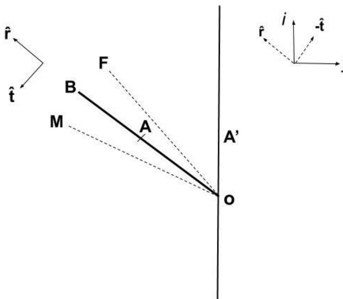
Fig. 2. \angle\text{FOM} represents the field of view of the observer O .
