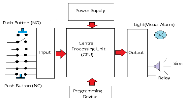
Block diagram of a PLC
