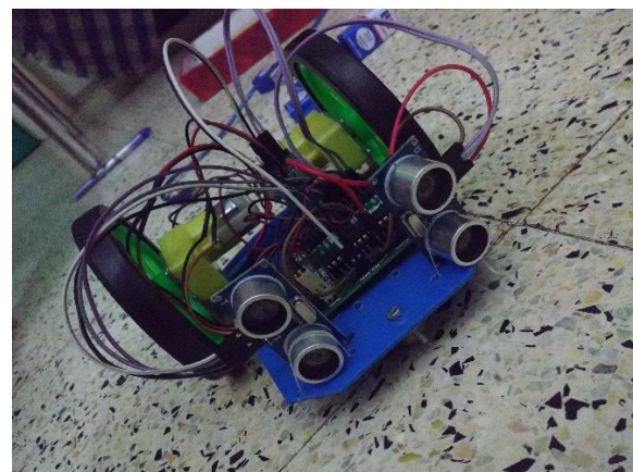
Fig.3. A smart robot car
