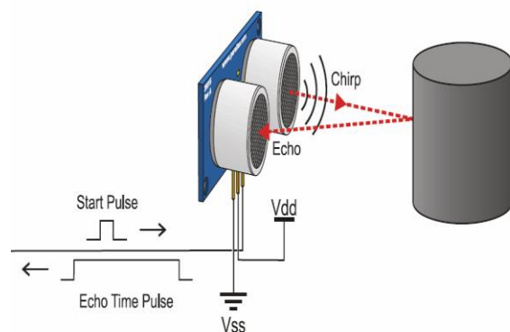
Fig. 4. Ultrasonic sensor
