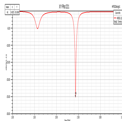
Fig: 10 optimized return loss of antenna
