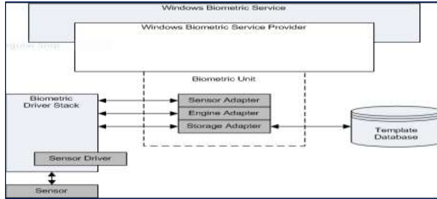
Figure 2: Biometric Framework
