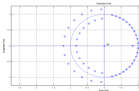
Fig. 3: Pole/Zero for Rectangular window.
