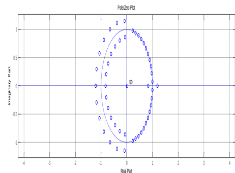
Fig. 6: Pole/Zero for Kaiser Window.
