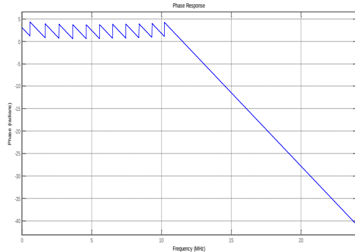
Fig. 2: Phase response for Rectangular window.
