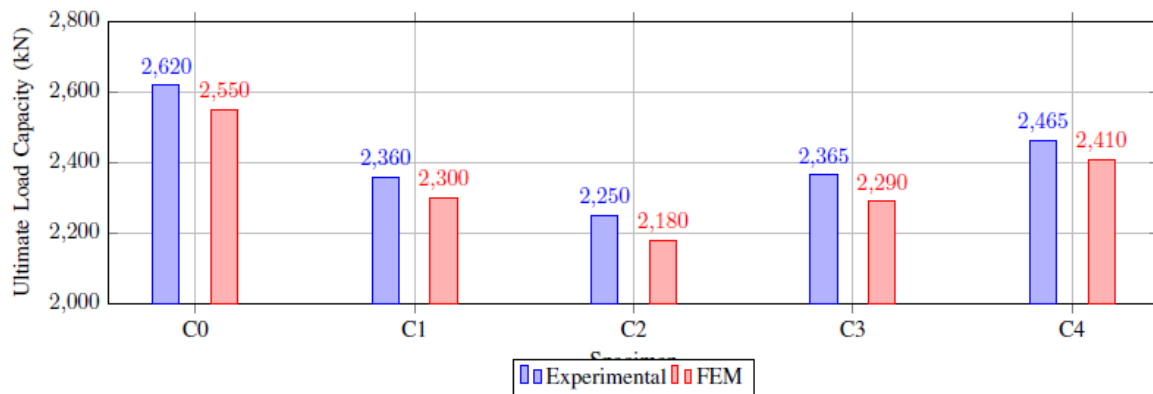
Fig. 4: Comparison of experimental vs FEM ultimate load capacity (illustrative).
