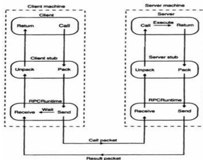
Fig2: RPC mechanism Implementation
