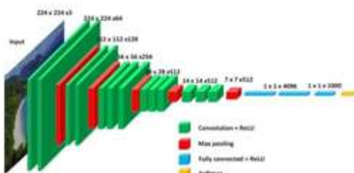
Figure 4 – VGG Model [17]
