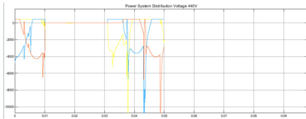
Fig 2. Three phase voltages when DSTATCOM is not connected to transmission lines and fault is introduced
