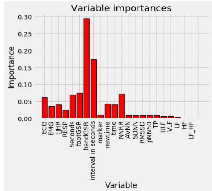
Fig 5. Variable Importances
