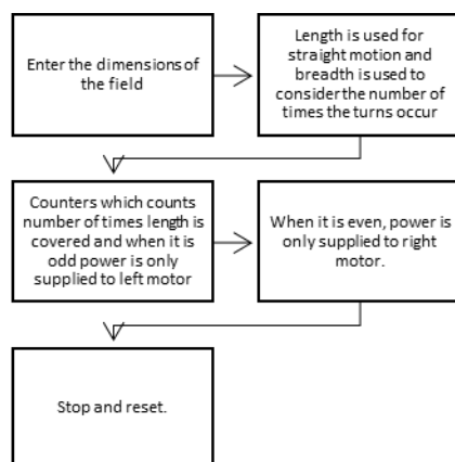
Fig 1: Flow Chart of Automation algorithm
