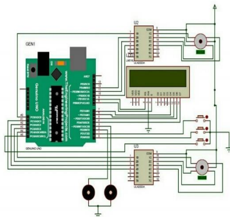
Fig 4: Internal circuit diagram
