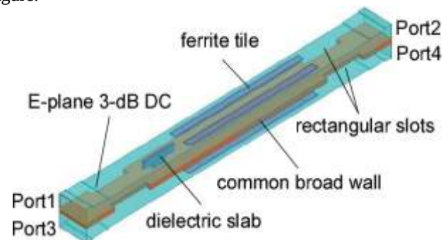
Fig. 2 Differential phase shift circulator with 90^\circ Phase shift
