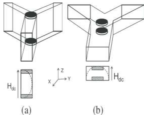
Fig.4: Waveguide Circulator
