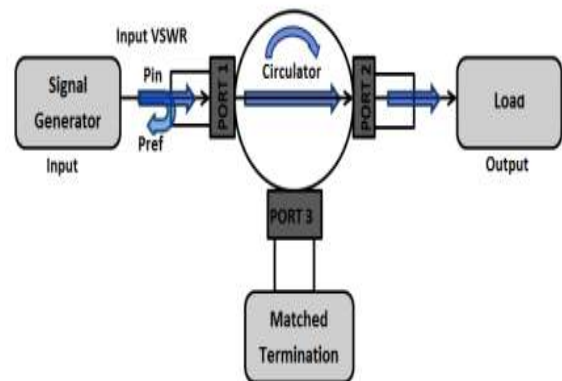
Fig 8: VSWR
