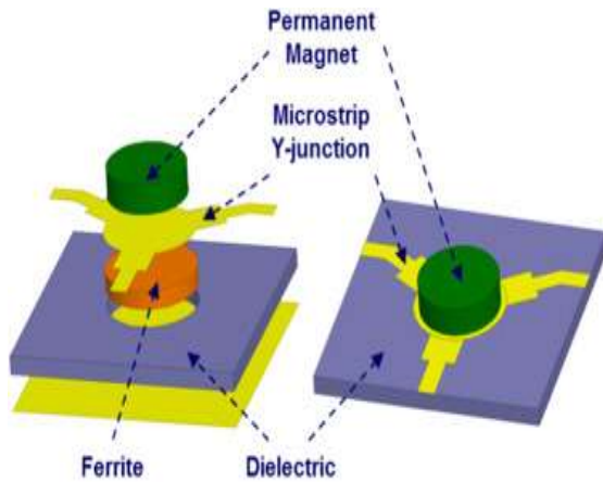
Fig.7: Strip-line Circulator
