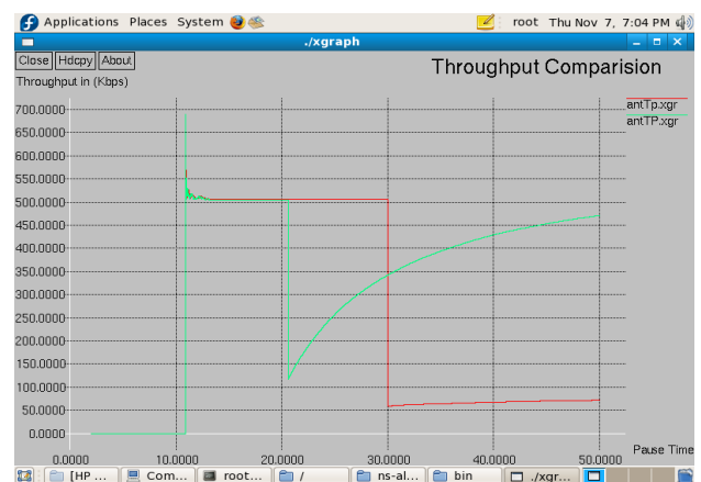
Figure: 5.4: Comparison of Ant & Novel Ant Algorithm in terms of Throughput.
