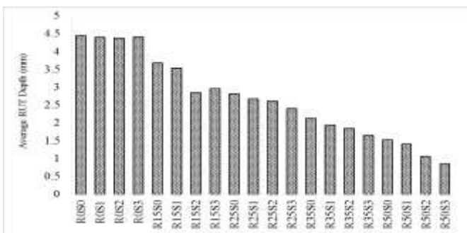
Fig. 7. Average Rut depth from HWTB testing
