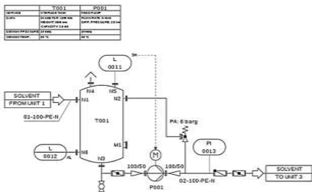
Figure 5 the Instrumentation Part of a Piping and Instrumentation Diagram
