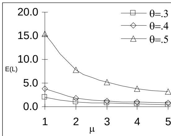
Fig. 4: Graph depicting the effect of \mu on E(L) by varying \theta .
