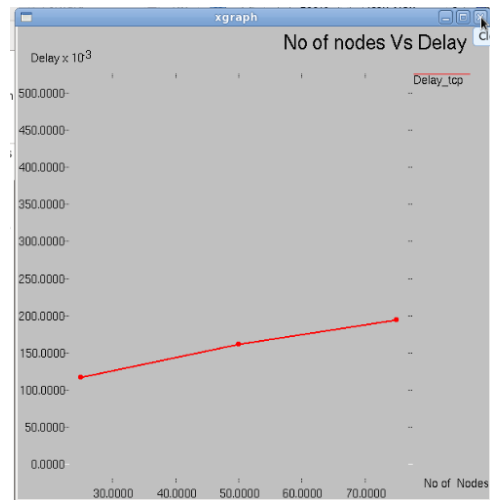
Figure 1: Graph of no. of nodes vs delay for mdp
