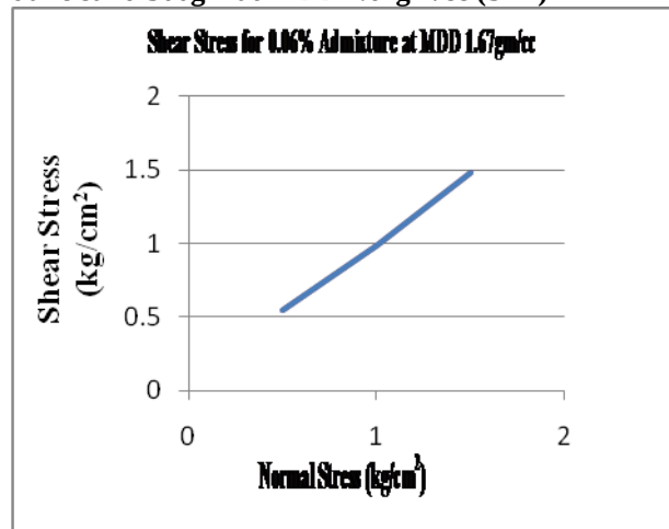
Figure shows 0.06% Admixture by wt that is 0.3gm + Dune sand 500gm at MDD 1.67gm/cc (SA2)
