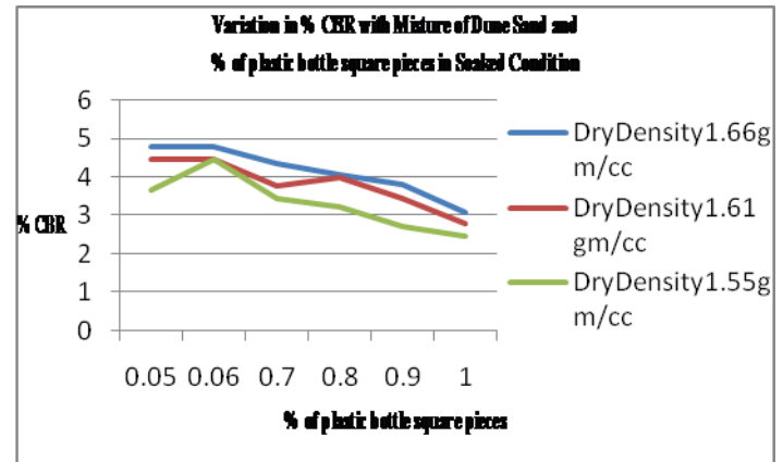
Figure shows variation in % CBR with mix of dune sand and % of plastic bottle square pieces in soaked condition
