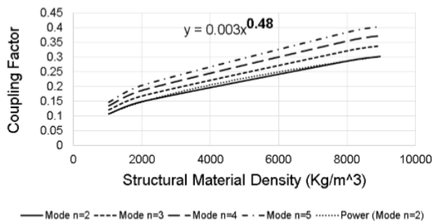
Figure 13. Effect of structural material density on coupling factor of water coupled cylinder with r/t = 250 - Cantilever boundary condition
