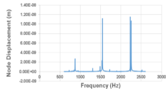
Figure 3: Frequency Response of Displacement of the Sphere - Solid Element
