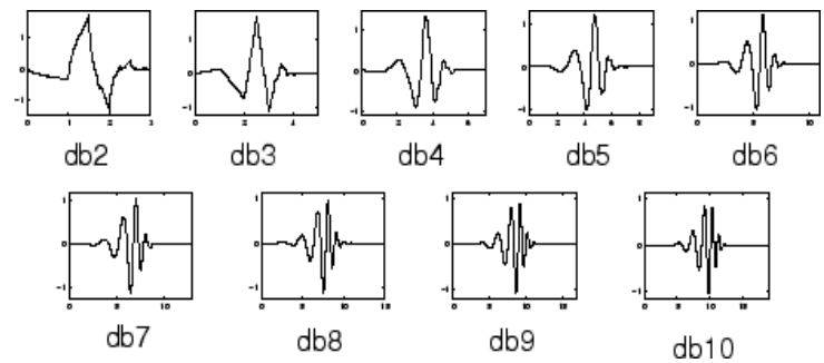
Fig 2: Daubechies wavelets
