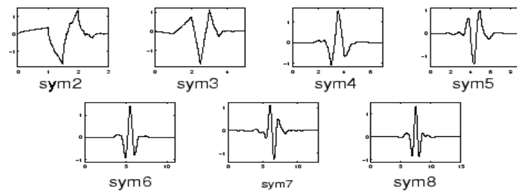
Fig 3: Symlet wavelets
