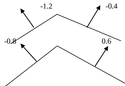
Figure- 3: Wind angle along purlin
