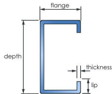
Figure-4: C section with lip
