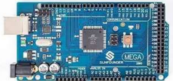
Figure 4: AT Mega 2560
