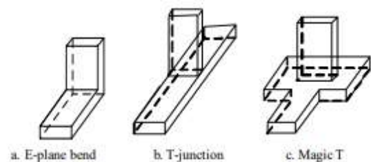
Fig.8 E-plane Structure
