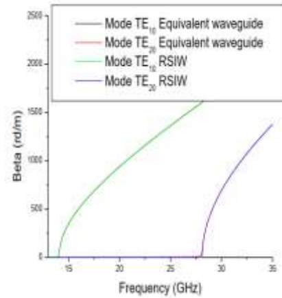
Fig.12 Dispersion characteristics.
