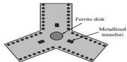
Fig.7 SIW Circulator
