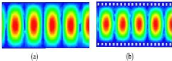
Fig.11 shows the electric field distribution of the TE 10 mode in the corresponding rectangular waveguide (a) and the RSIW (b) at f = 22GHz.
