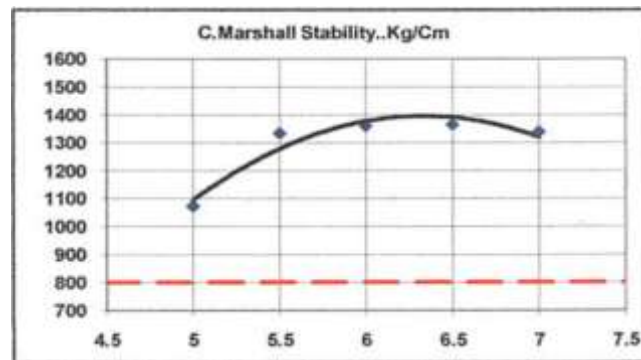
Graph 1. Marshall Stability
